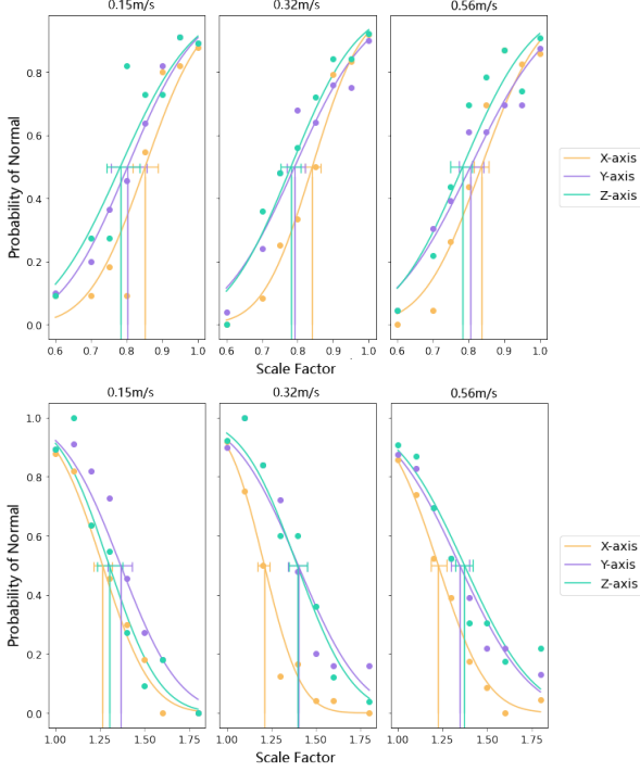
Figure 3. Fitted logistic functions for each speed level, paired by the axis of movement. Dropdown lines mark the threshold point. Error bars indicate 95% confidence intervals expressed in Table 1.
